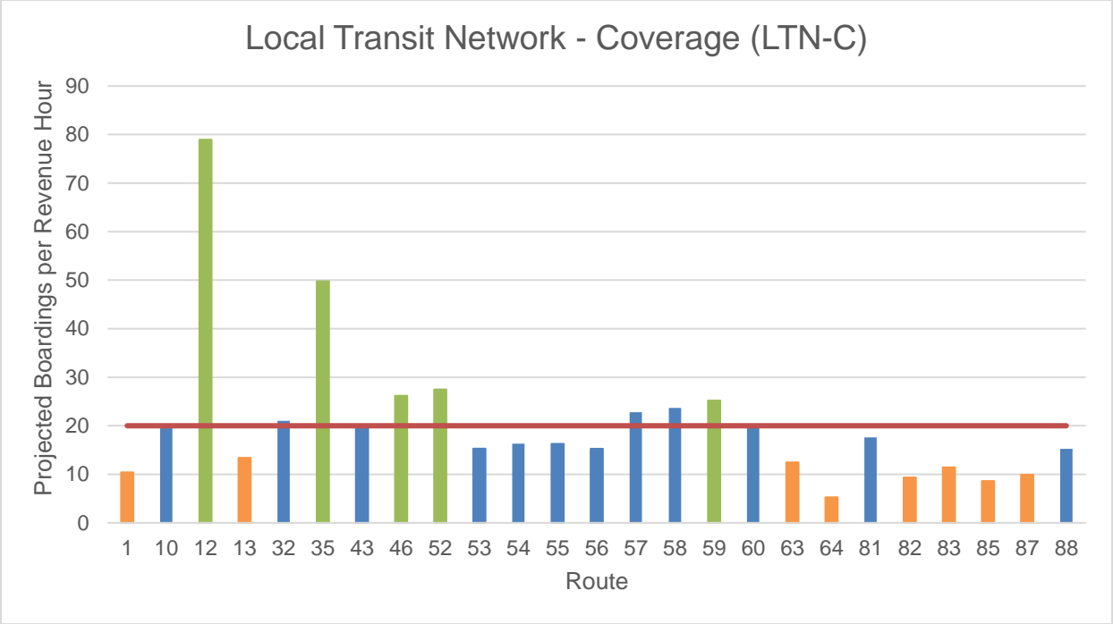
Figure 4: Projected Boardings per Revenue Hour for the Local Transit Network - Coverage, Fall 2022 (Performance Guideline = 20)
