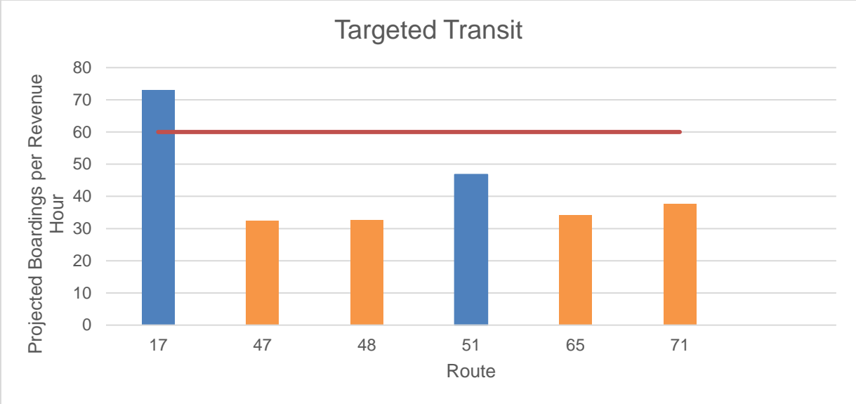
Figure 5: Projected Boardings per Revenue Hour for Targeted Transit, Fall 2022 (Performance Guideline = 60)
